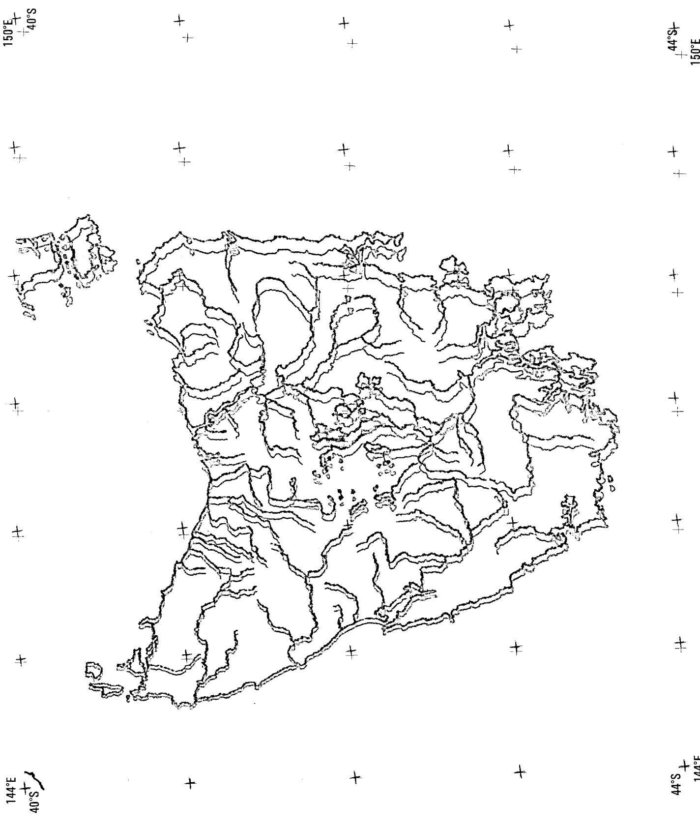
FIGURE 3.1 COMPARISON OF LAMBERT CONFORMAL AND SIMPLE CONIC MAP PROJECTION
