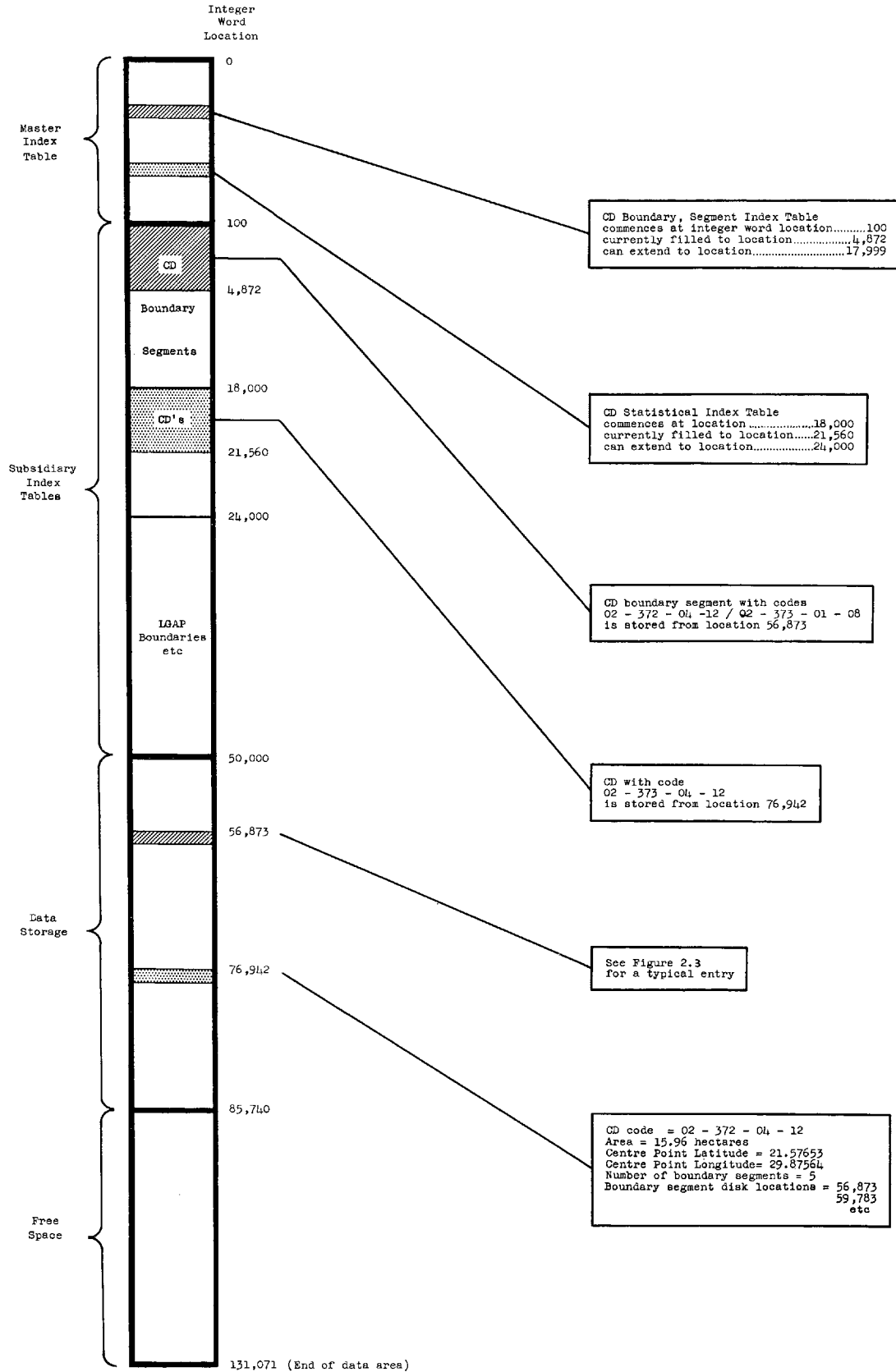
Figure 2.7 : Disk data structure.
